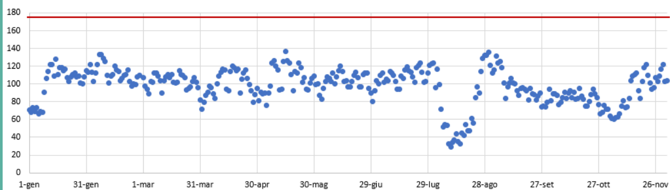
COD (mg/l)
